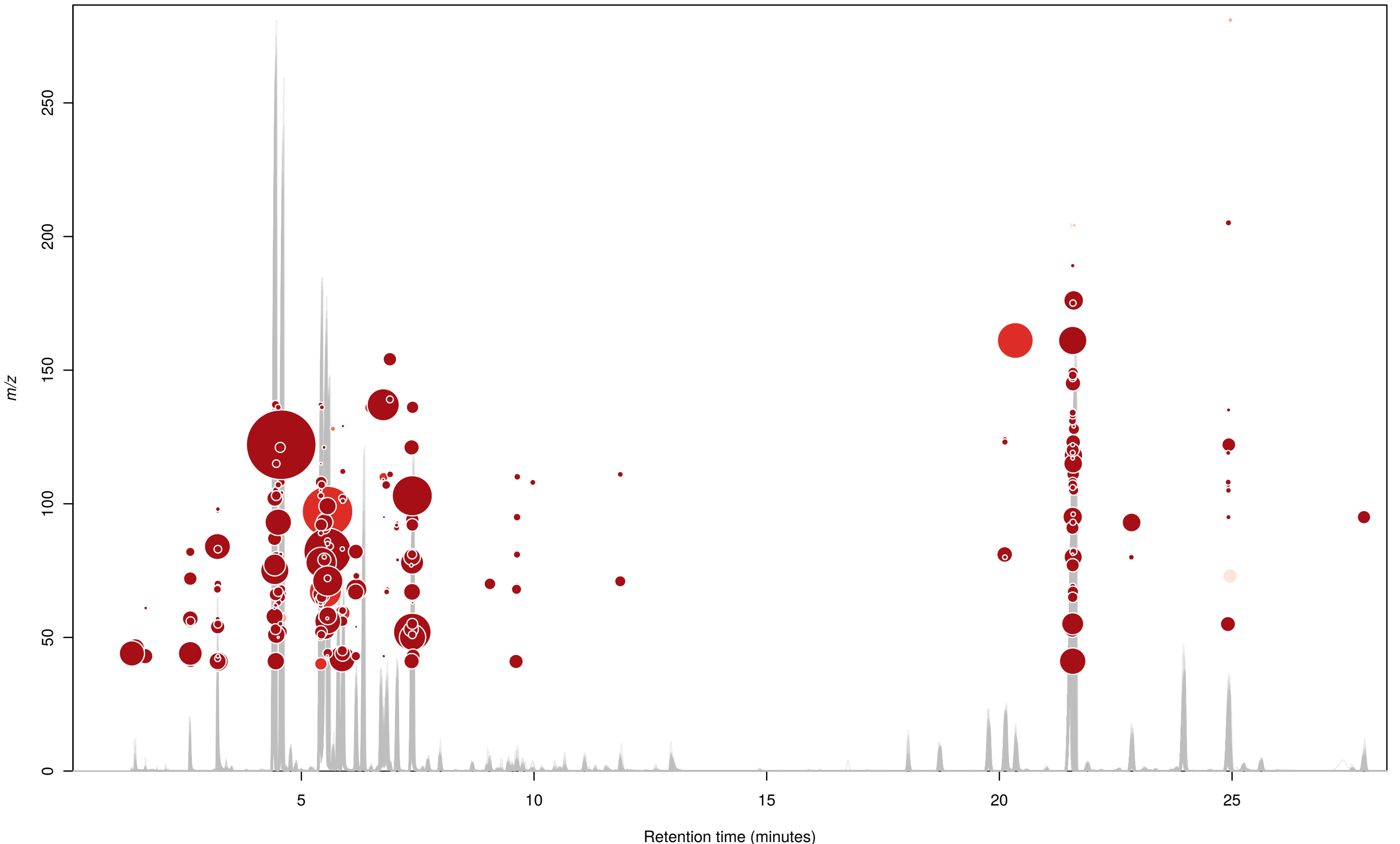
Cloud Plot 285 features with p-value \leq 0.01
