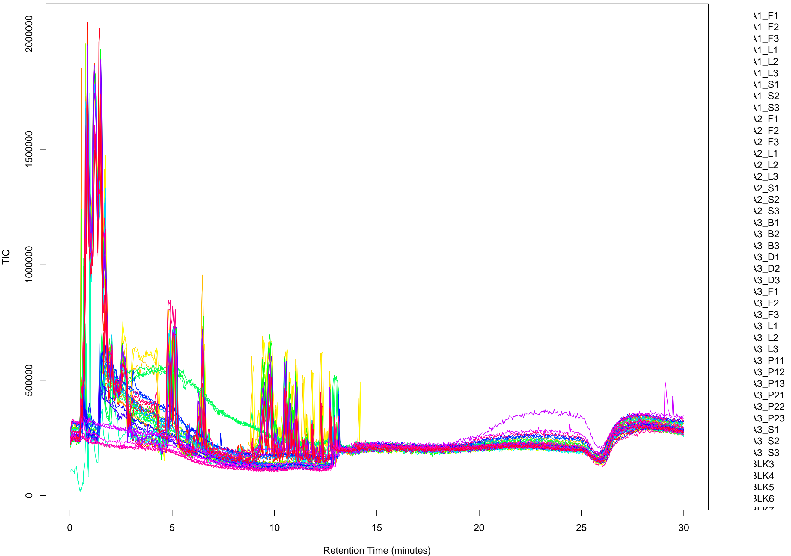
Total Ion Chromatograms (original)
